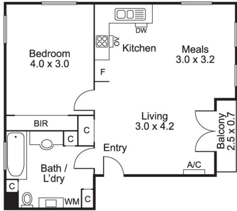
SIXTH FLOOR
