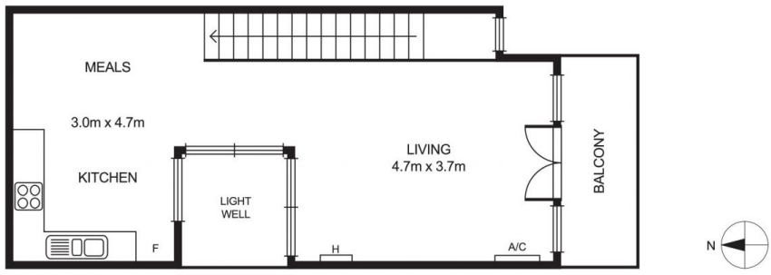
UPPER LEVEL
